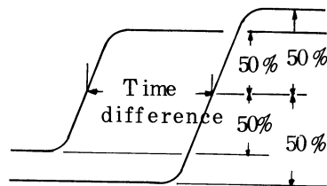
Measuring method by super position
